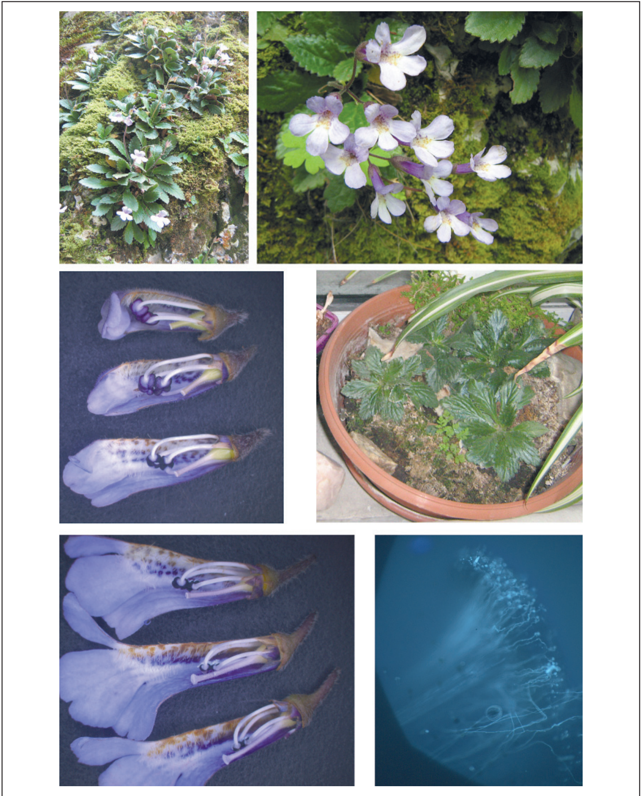
Plate I. Fig. 1. Typical microhabitat of Haberlea rhodopensis ; Fig. 2. The flowers bear features of bee pollination syndrome; Figs 3 and 5. Floral mechanism – weak protandry and strong herkogamy; Fig. 4. Plants transferred in spring and early summer, especially if taken with the moss cushion, were doing very well ex situ ; Fig. 6. Pollen tube growth.
