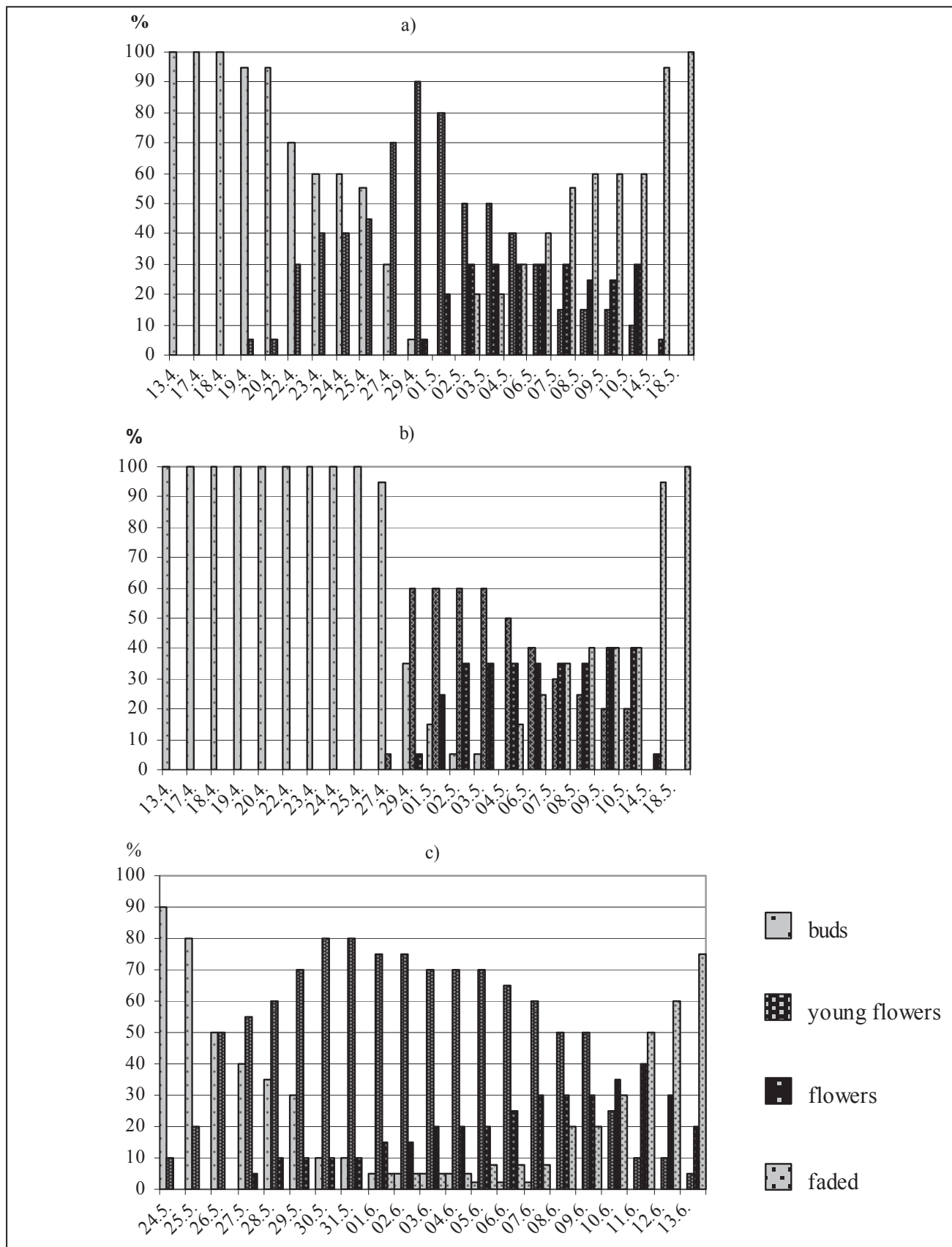
Fig. 1. Comparative phenology of three sites: a) population exposed to sunshine from the Botanical Garden of Mainz University, 100 m a.s.l.; b) population in shadow from the Botanical Garden of Mainz University; c) natural population in Ustovo district, Central Rhodopi, 800 m a.s.l.
