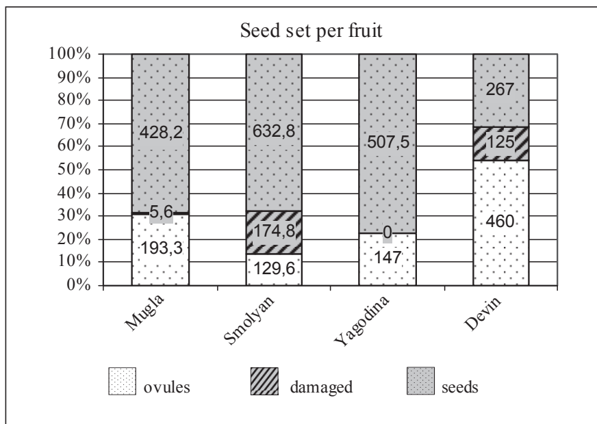
Fig. 2. Seed set per capsule of random samples from four different natural populations in the Central Rhodopi Mountains.
