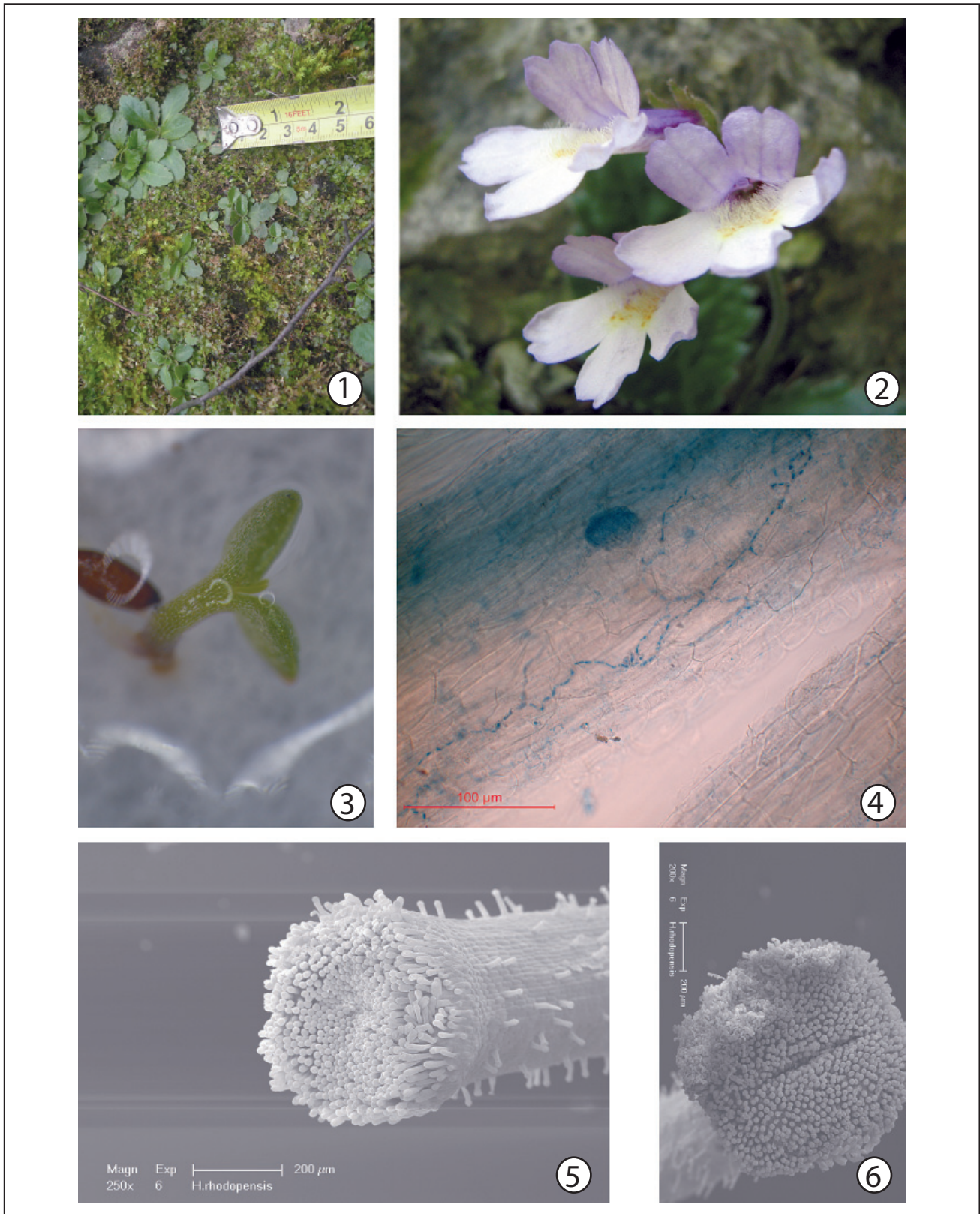
Plate II. Fig. 1. Haberlea rhodopensis has good ability for vegetative propagation; Fig. 2. The flowers bear features of bee pollination syndrome; Fig. 3. Seedling of age about four five months; Fig. 4. Root microscope preparations clearly show the structures, which indicate the mycorrhiza; Figs 5 and 6. Changes in the stigma area indicating receptivity are visible on the microscopic pictures.
